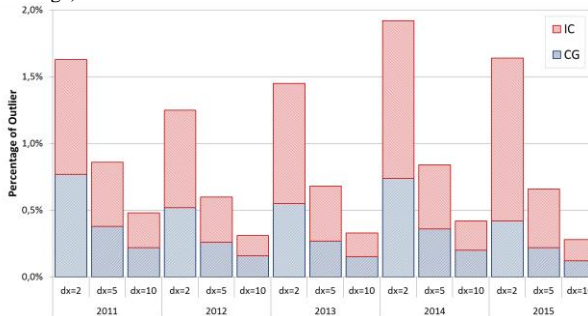
Fig. 4b: Percentage of outliers in Belgium (inside the weather radar coverage)
